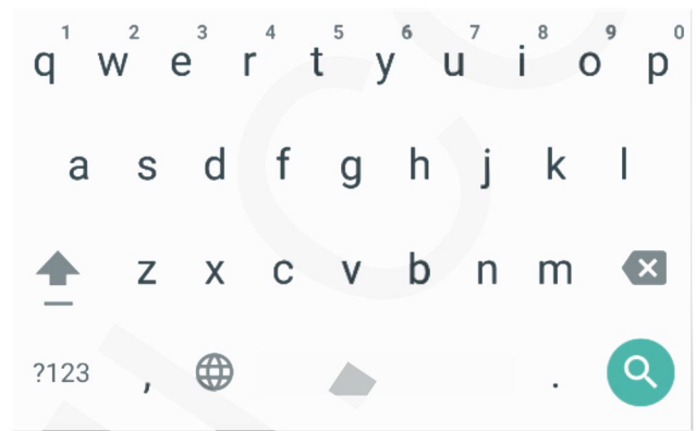
Google Keyboard
